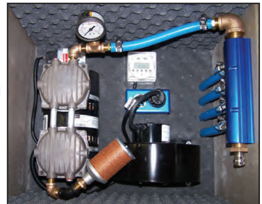
Compression Unit
